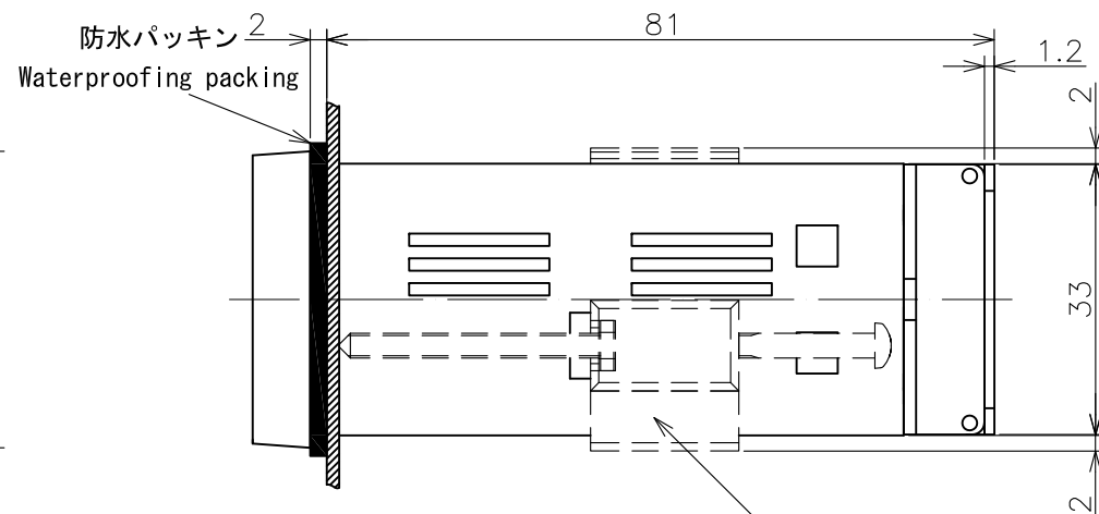
取付具 (固定ネジ: M3) Fixture (Fixed screw: M3)
