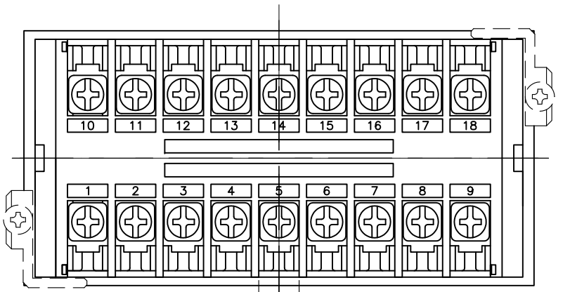
端子ネジ: M3.5 Terminal screws: M3.5
