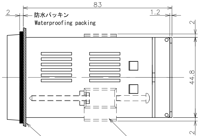
取付具 (固定ネジ: M3) Fixture (Fixed screw: M3)
